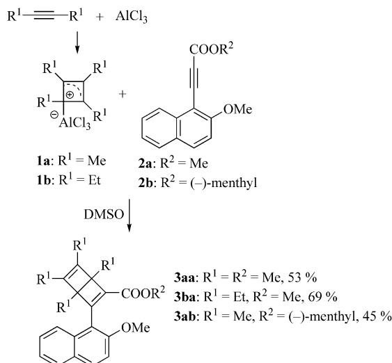
Scheme 1. Formation 2-methoxy-1-naphthyl-substituted Dewar benzenes 3 .
