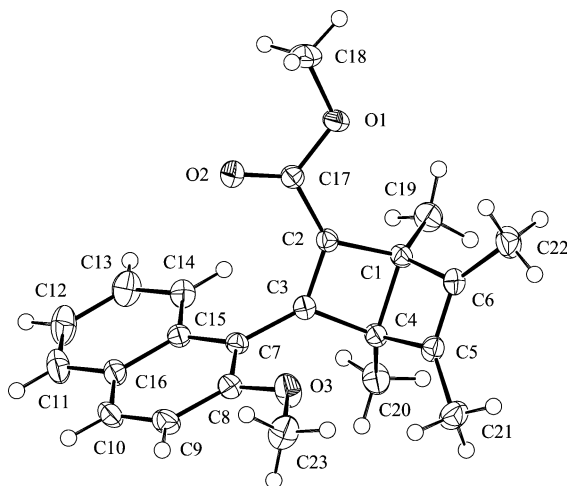
Figure 1. X-ray structure of 3aa . Displacement parameters are shown at the 50% probability level.
