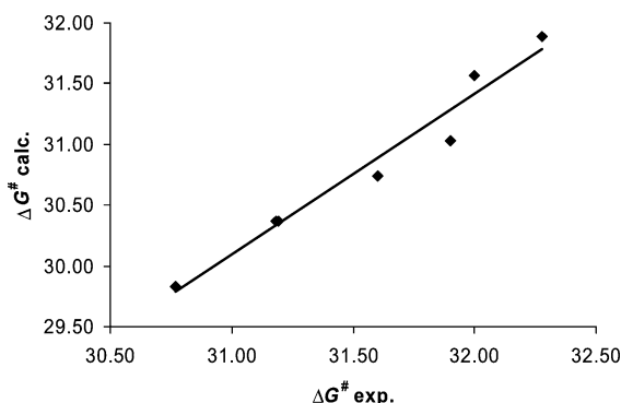
Figure 4. Correlation between calculated and experimental free energies of activation of Dewar benzene derivatives rearrangement.
