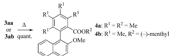
Scheme 2. Rearrangement of 3aa and 3ab into benzenes 4 .
