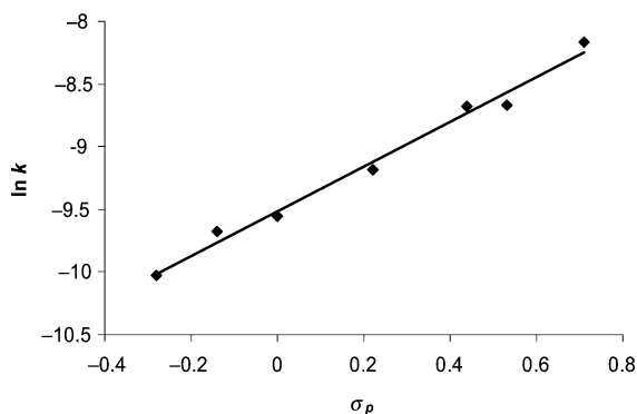
Figure 3. Correlation of para - \sigma Hammett constants with \ln of rearrangement rate constants k .
