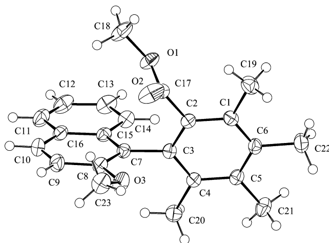
Figure 2. X-ray structure of 4a . Displacement parameters are shown at the 50% probability level.
